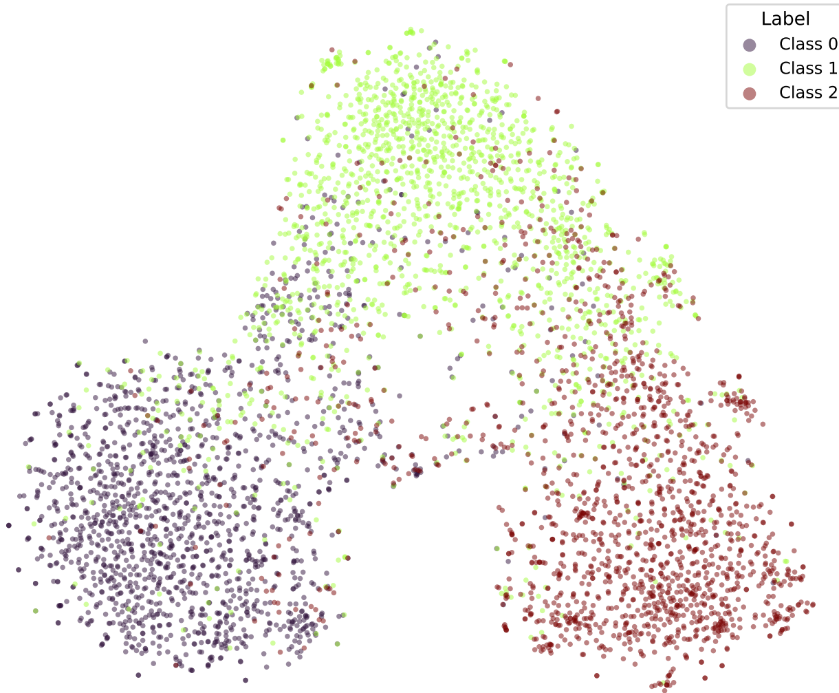
google/bert_uncased_L-2_H-128_A-2-snli-SOFT3-TRIPa2-1 (val)
