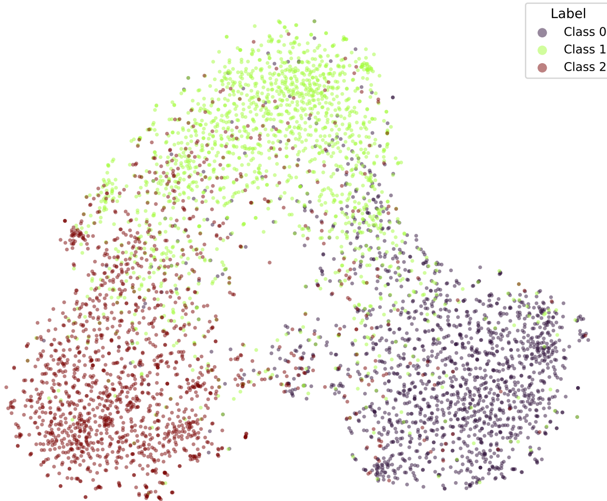
google/bert_uncased_L-2_H-128_A-2-snli-SOFT3-TRIPa2-4 (val)
