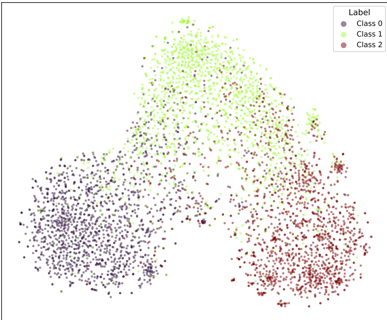
google/bert_uncased_L-2_H-128_A-2-snli-SOFT4-TRIPa1-1 (val)
