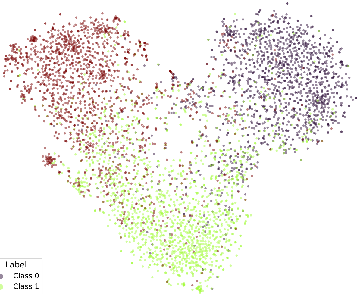
google/bert_uncased_L-2_H-128_A-2-snli-SOFT4-TRIPa1-2 (val)
