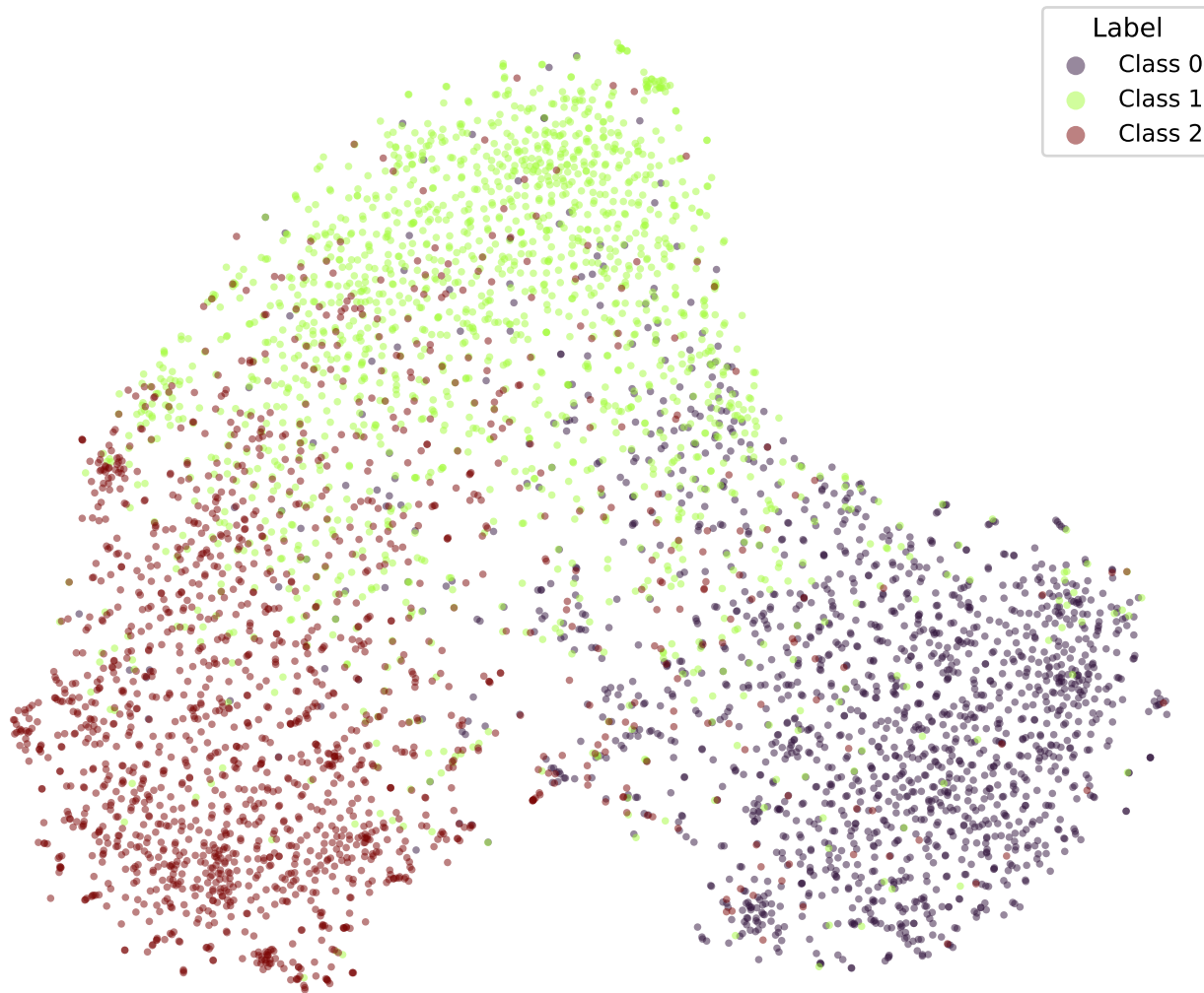
google/bert_uncased_L-2_H-128_A-2-snli-SOFT4-TRIPa1-4 (val)
