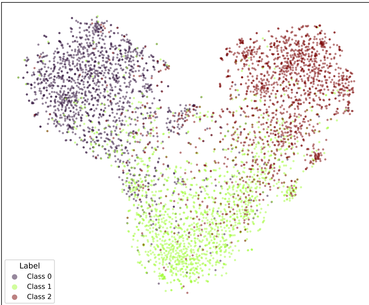
google/bert_uncased_L-2_H-128_A-2-snli-SOFT4-TRIPa2-3 (val)
