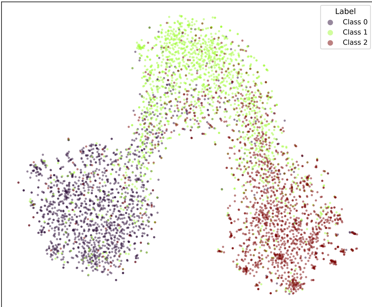
google/bert_uncased_L-2_H-128_A-2-snli-WKL-TRIPa1-2 (val)
