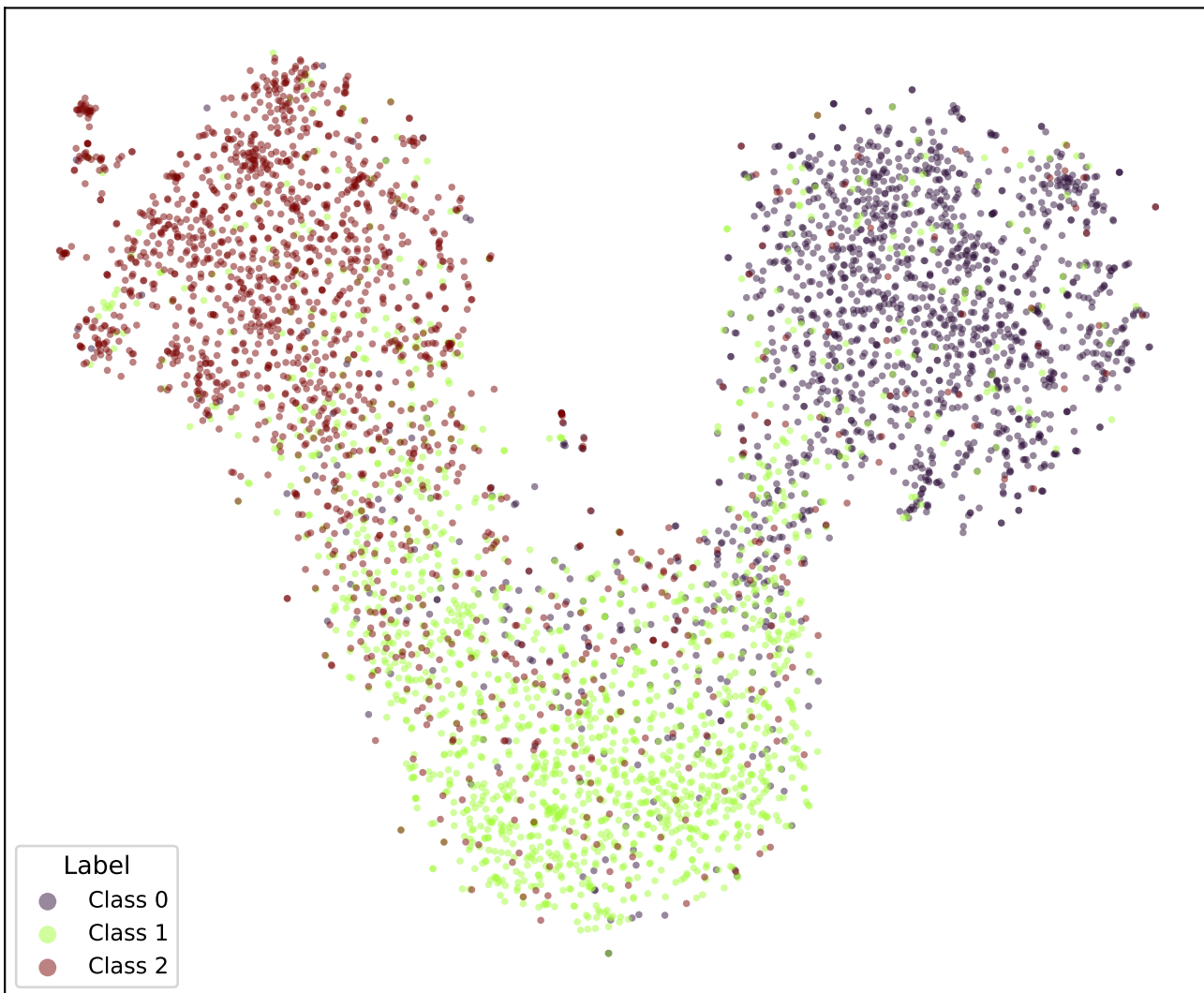
google/bert_uncased_L-2_H-128_A-2-snli-WKL-TRIPa1-3 (val)
