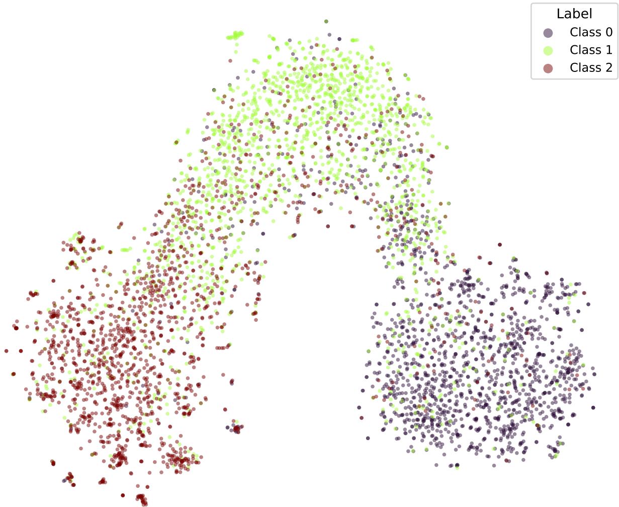
google/bert_uncased_L-2_H-128_A-2-snli-WKL-TRIPa1-5 (val)
