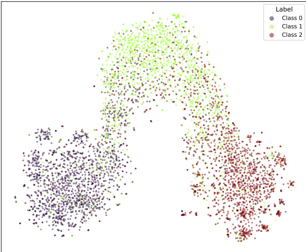
google/bert_uncased_L-2_H-128_A-2-snli-WKL-TRIPa2-5 (val)
