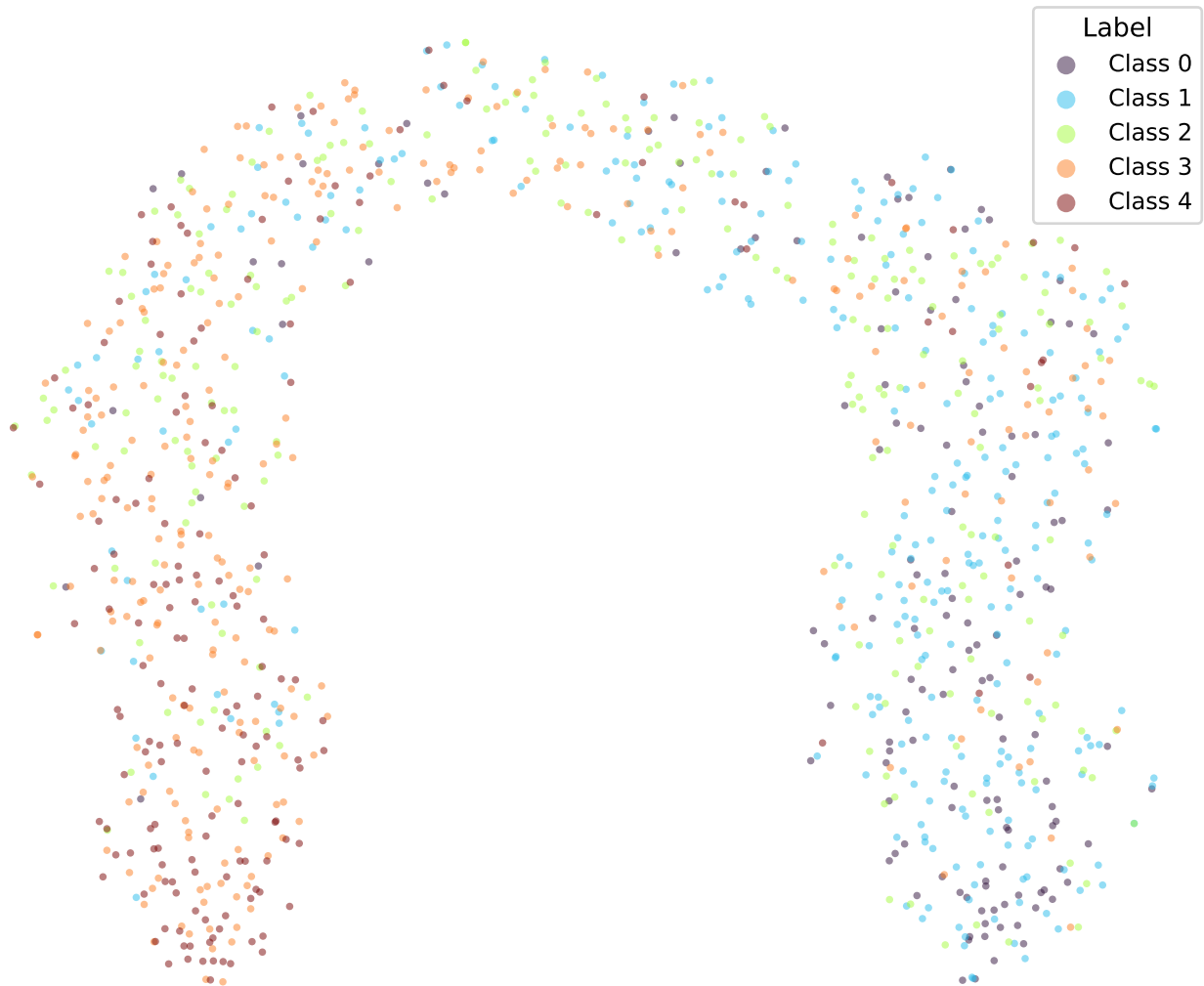
google/bert_uncased_L-2_H-128_A-2-sst5-BCE-TRIPa1-1 (val)
