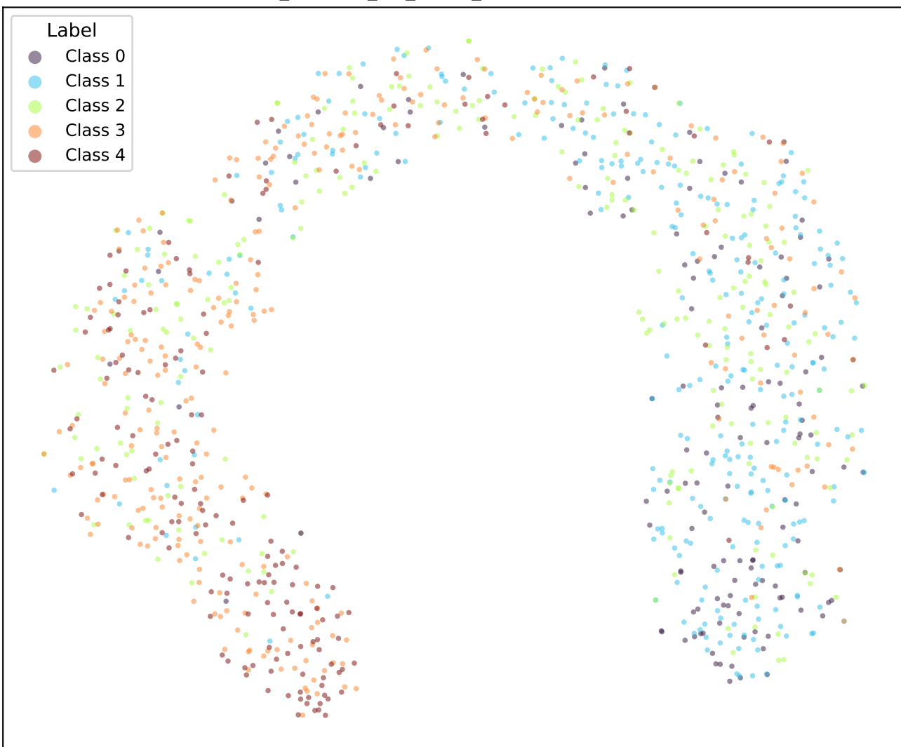
google/bert_uncased_L-2_H-128_A-2-sst5-BCE-TRIPa1-4 (val)
