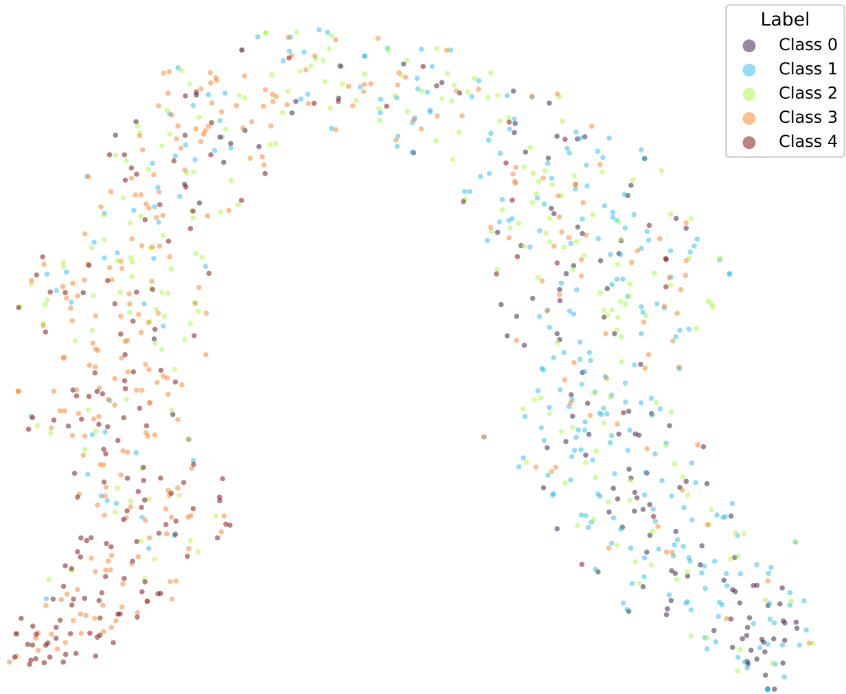
google/bert_uncased_L-2_H-128_A-2-sst5-BCE-TRIPa2-1 (val)
