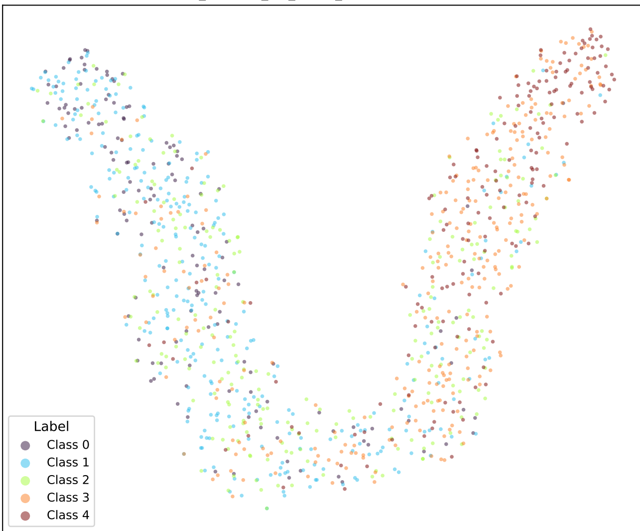
google/bert_uncased_L-2_H-128_A-2-sst5-BCE-TRIPa2-2 (val)
