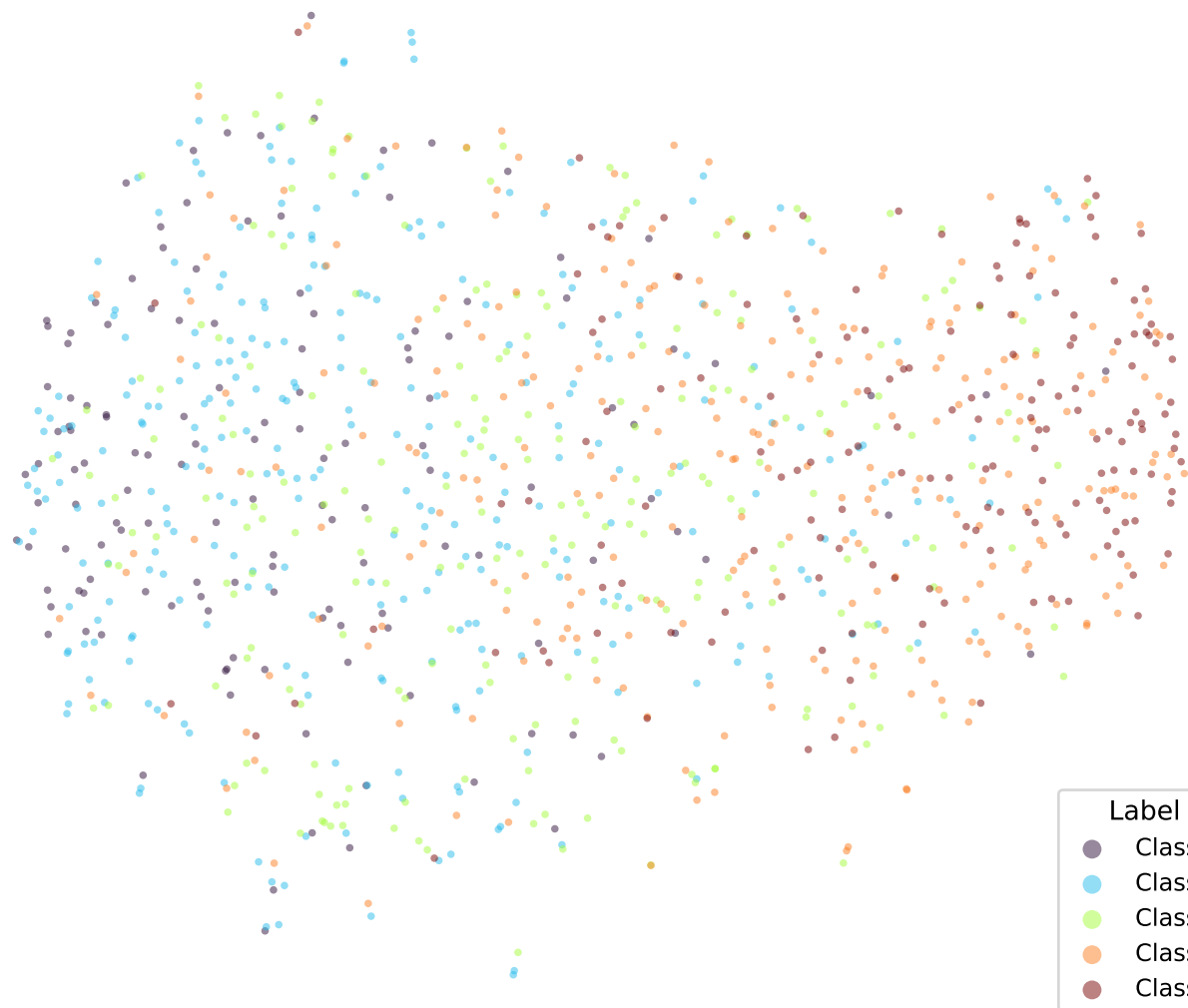
google/bert_uncased_L-2_H-128_A-2-sst5-CE-TRIPa1-1 (val)
