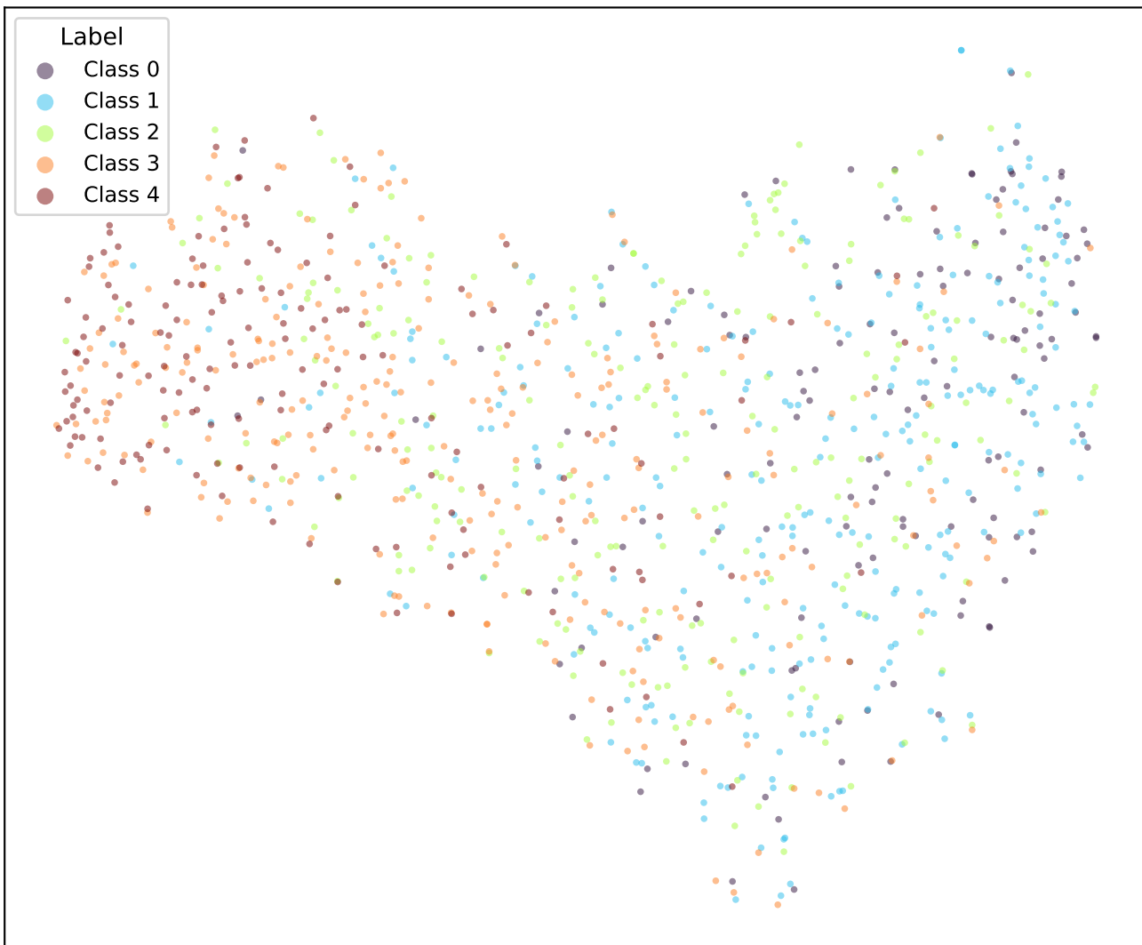
google/bert_uncased_L-2_H-128_A-2-sst5-CE-TRIPa1-3 (val)
