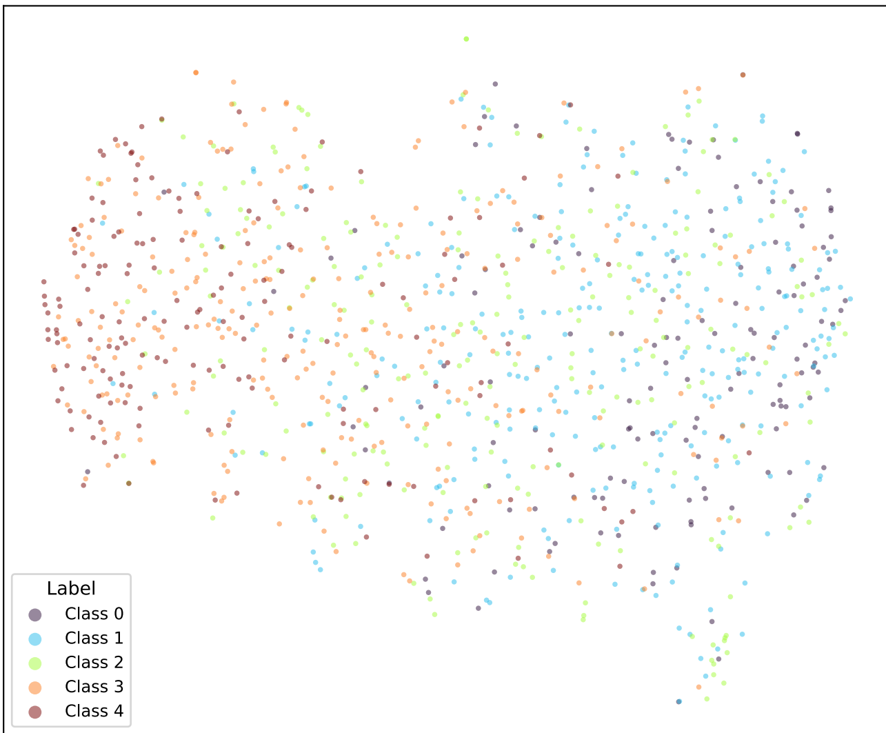
google/bert_uncased_L-2_H-128_A-2-sst5-CE-TRIPa1-5 (val)
