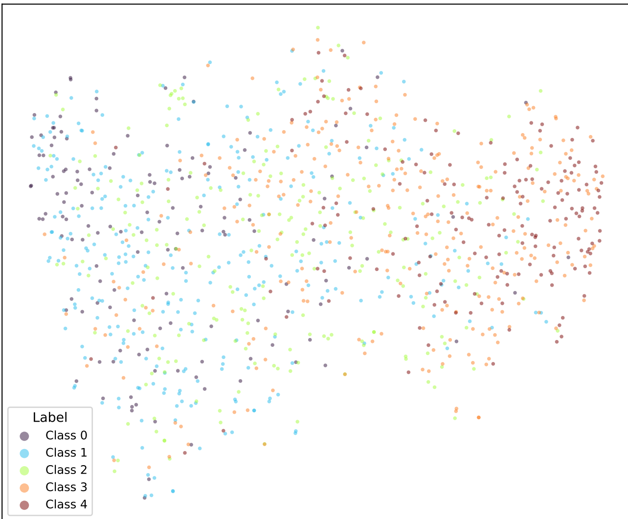
google/bert_uncased_L-2_H-128_A-2-sst5-CE-TRIPa2-1 (val)
