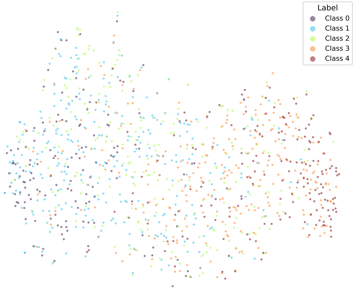
google/bert_uncased_L-2_H-128_A-2-sst5-CE-TRIPa2-2 (val)
