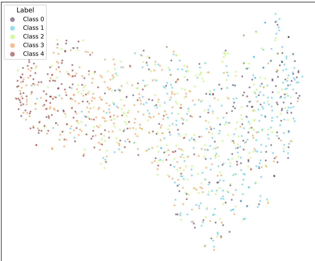
google/bert_uncased_L-2_H-128_A-2-sst5-CE-TRIPa2-3 (val)
