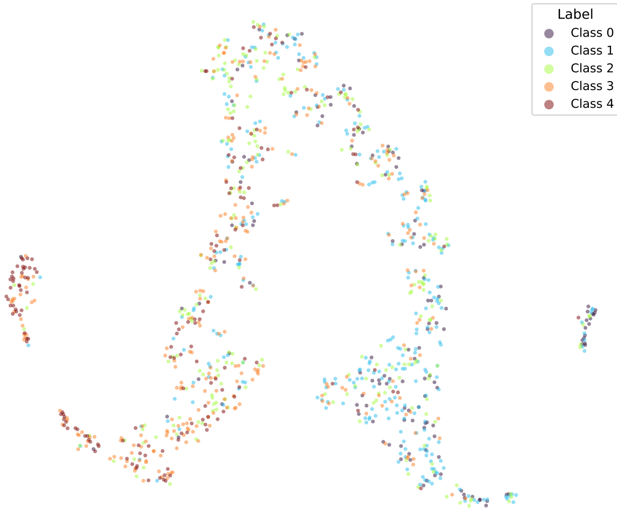
google/bert_uncased_L-2_H-128_A-2-sst5-CORAL-TRIPa1-2 (val)
