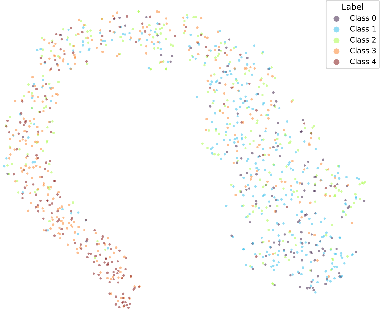
google/bert_uncased_L-2_H-128_A-2-sst5-CORN-4 (val)
