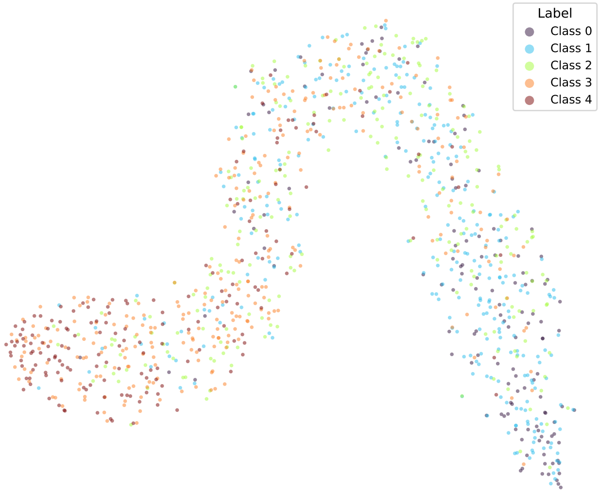
google/bert_uncased_L-2_H-128_A-2-sst5-CORN-5 (val)
