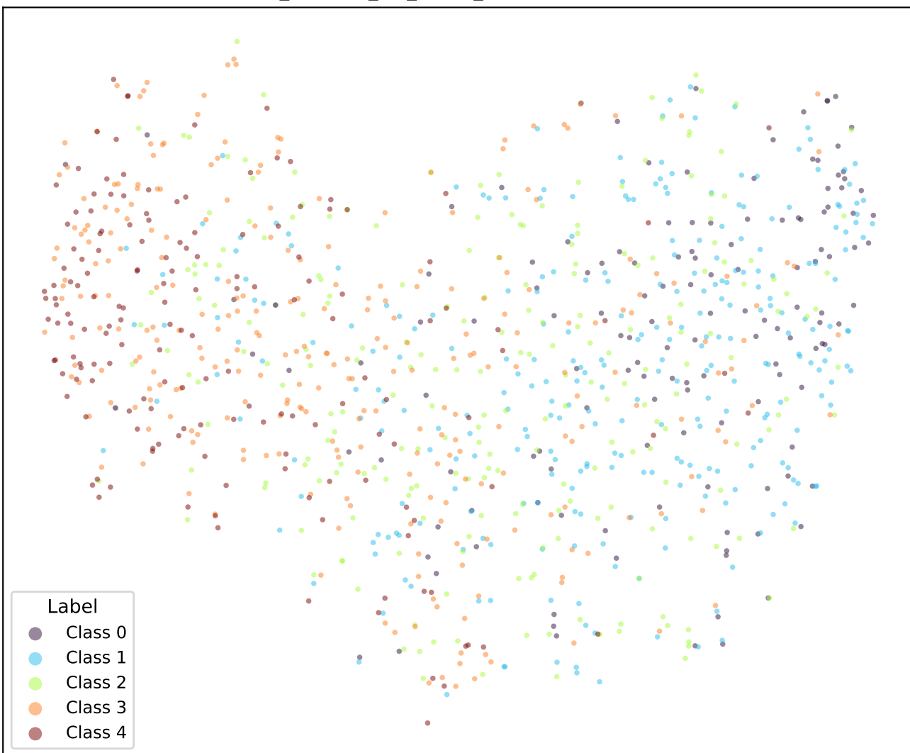
google/bert_uncased_L-2_H-128_A-2-sst5-EMD-TRIPa1-1 (val)
