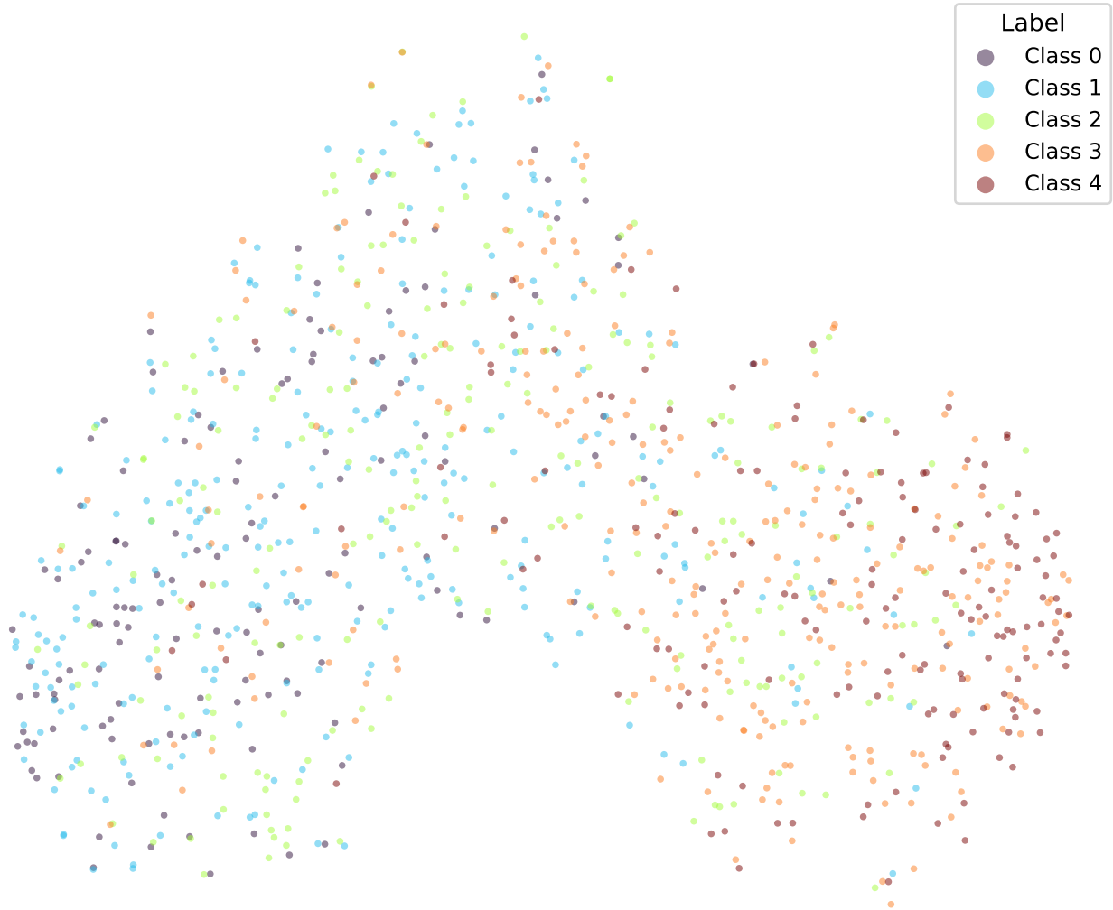
google/bert_uncased_L-2_H-128_A-2-sst5-EMD-TRIPa1-2 (val)
