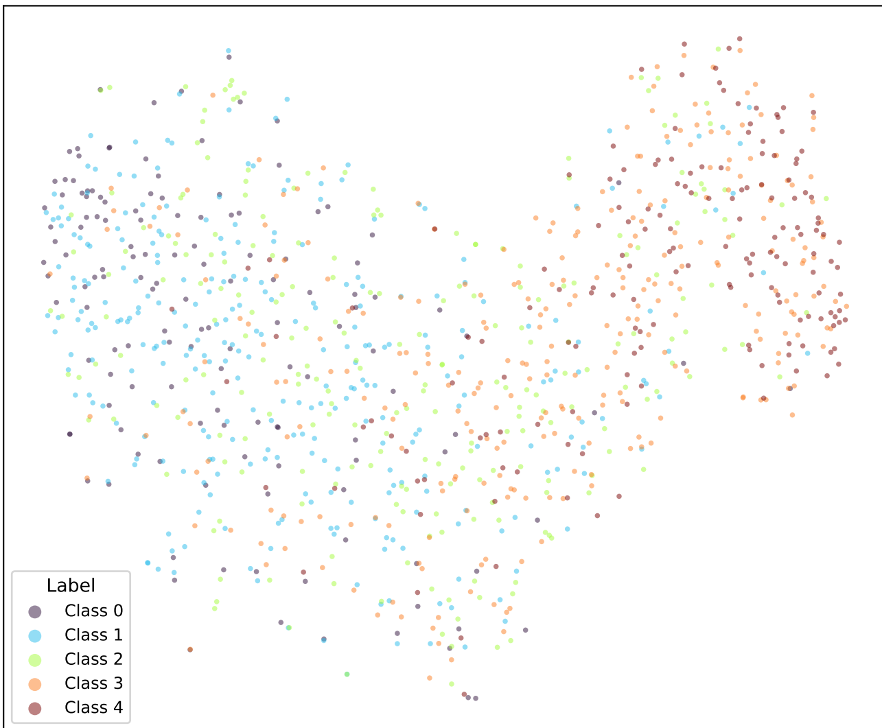
google/bert_uncased_L-2_H-128_A-2-sst5-EMD-TRIPa1-3 (val)
