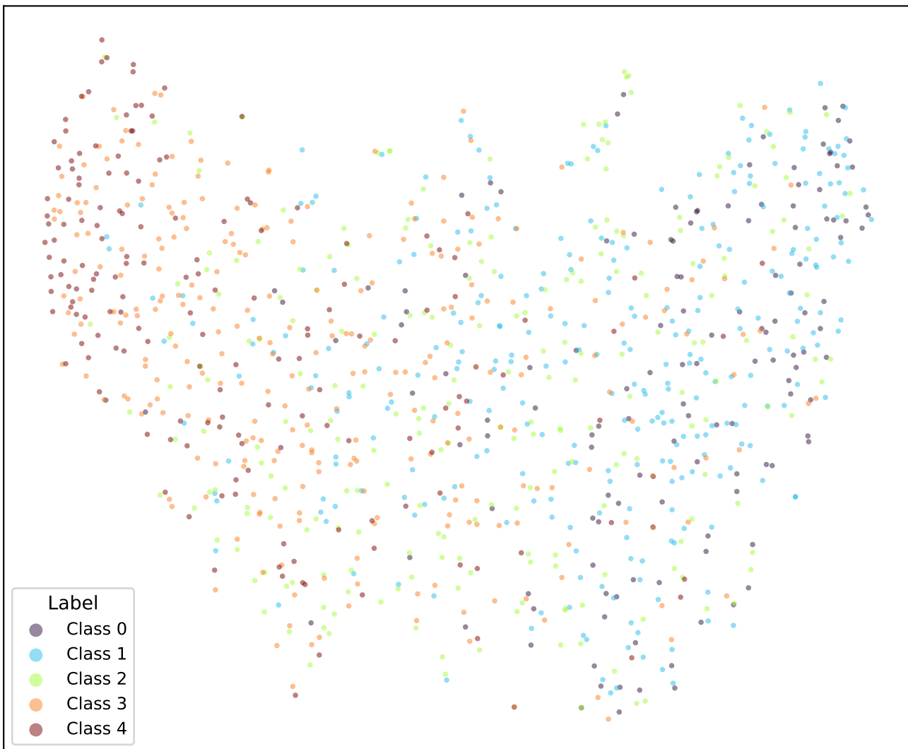
google/bert_uncased_L-2_H-128_A-2-sst5-EMD-TRIPa1-5 (val)
