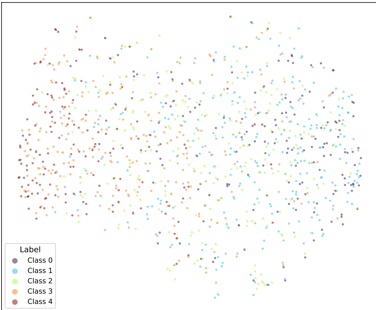
google/bert_uncased_L-2_H-128_A-2-sst5-EMD-TRIPa2-1 (val)
