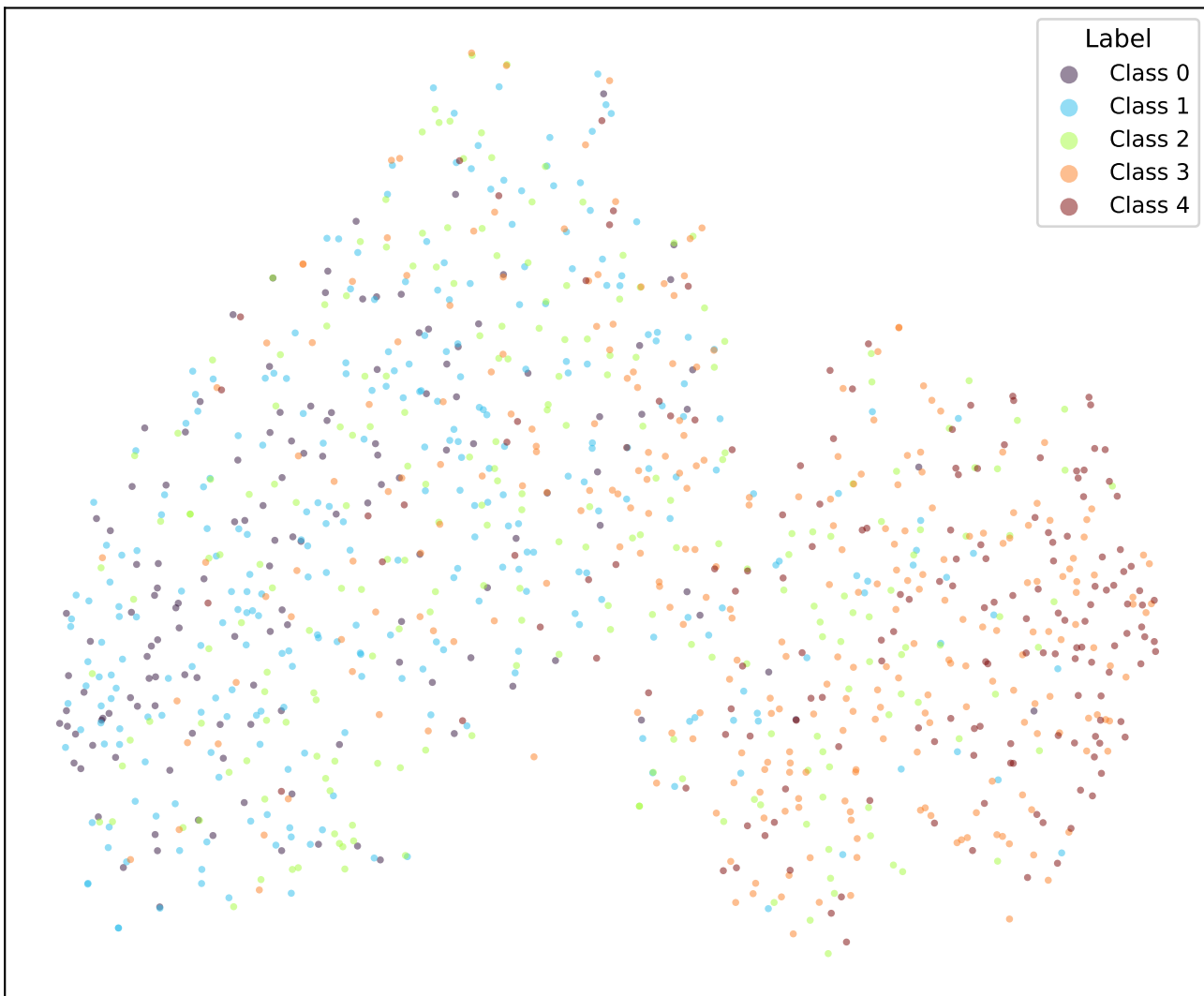
google/bert_uncased_L-2_H-128_A-2-sst5-EMD-TRIPa2-2 (val)
