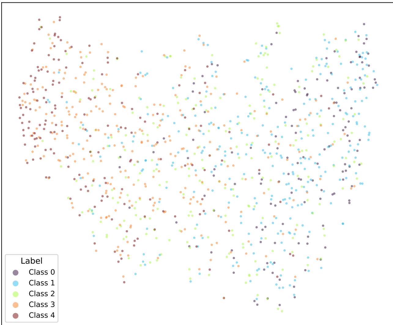
google/bert_uncased_L-2_H-128_A-2-sst5-EMD-TRIPa2-5 (val)
