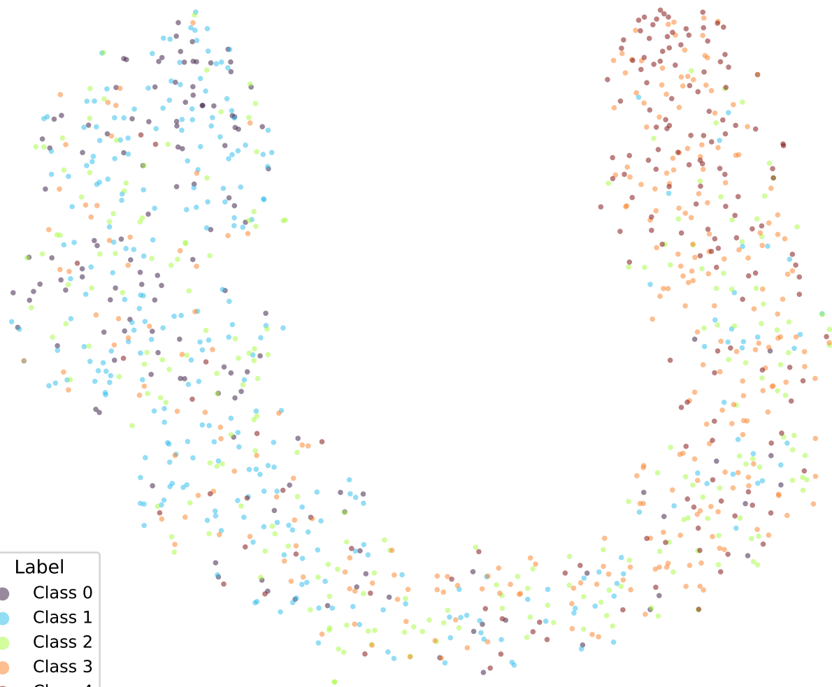
google/bert_uncased_L-2_H-128_A-2-sst5-OLL1-TRIPa2-5 (val)
