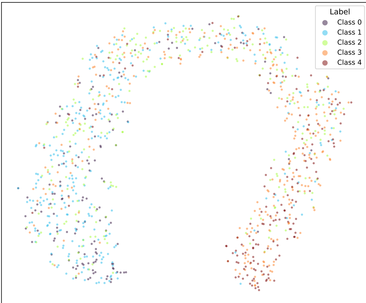
google/bert_uncased_L-2_H-128_A-2-sst5-OLL15-TRIPa1-1 (val)
