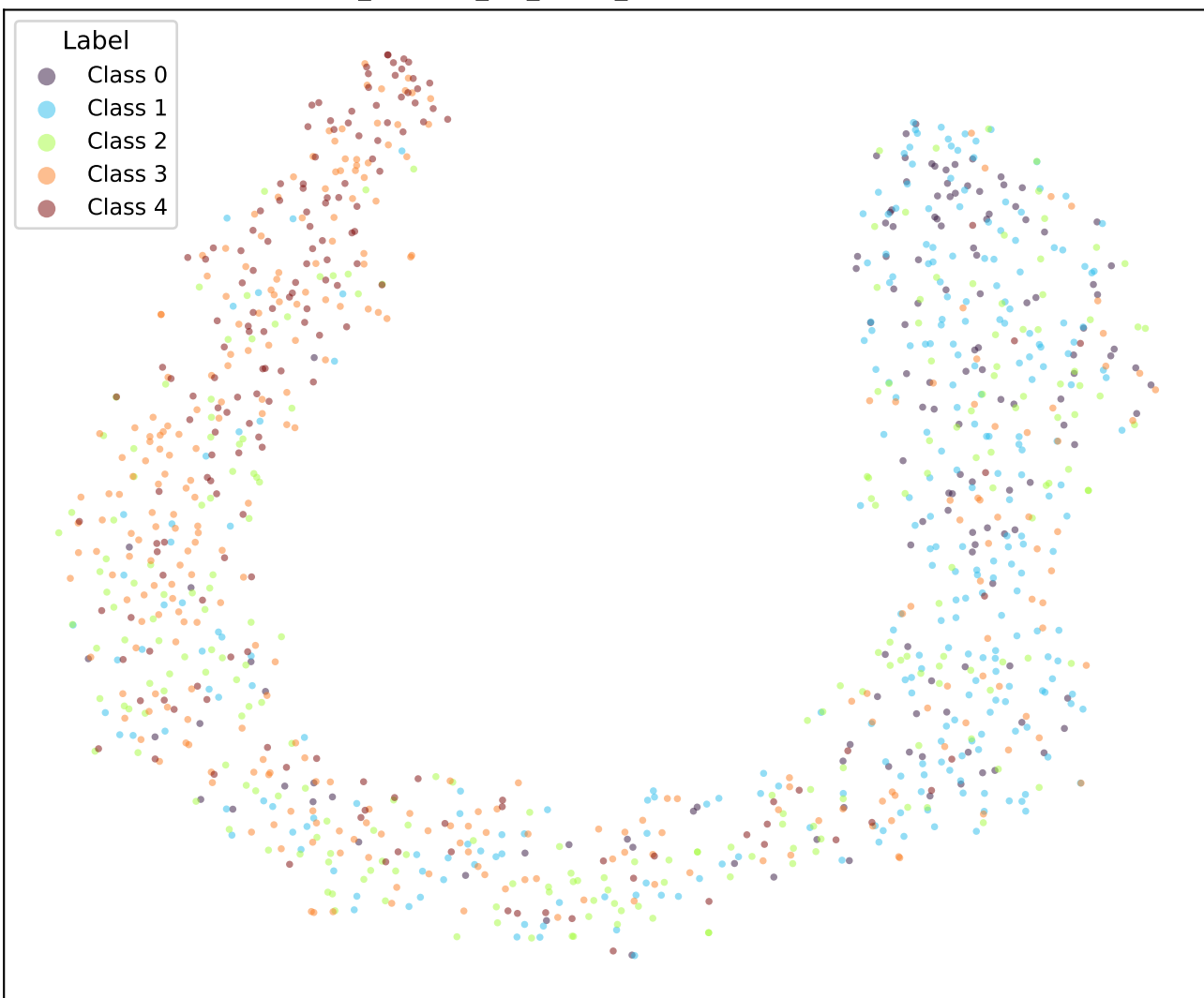
google/bert_uncased_L-2_H-128_A-2-sst5-OLL15-TRIPa2-5 (val)
