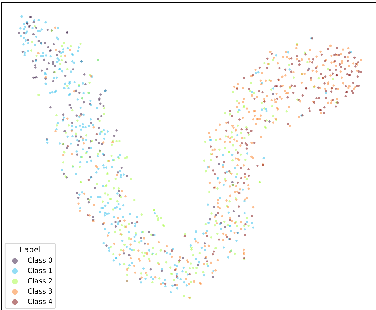
google/bert_uncased_L-2_H-128_A-2-sst5-OLL2-TRIPa1-4 (val)
