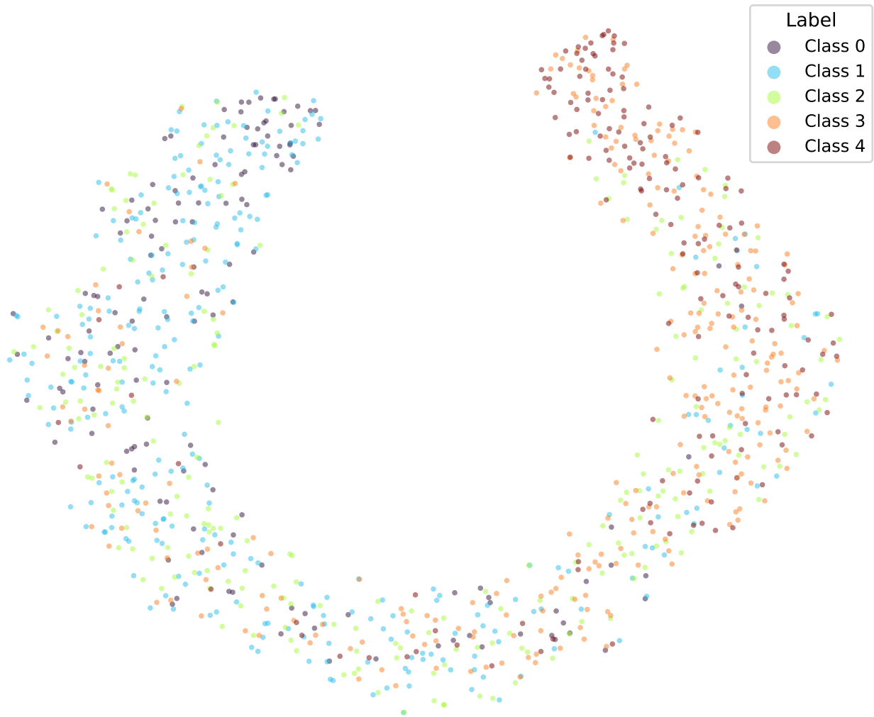
google/bert_uncased_L-2_H-128_A-2-sst5-OLL2-TRIPa2-2 (val)
