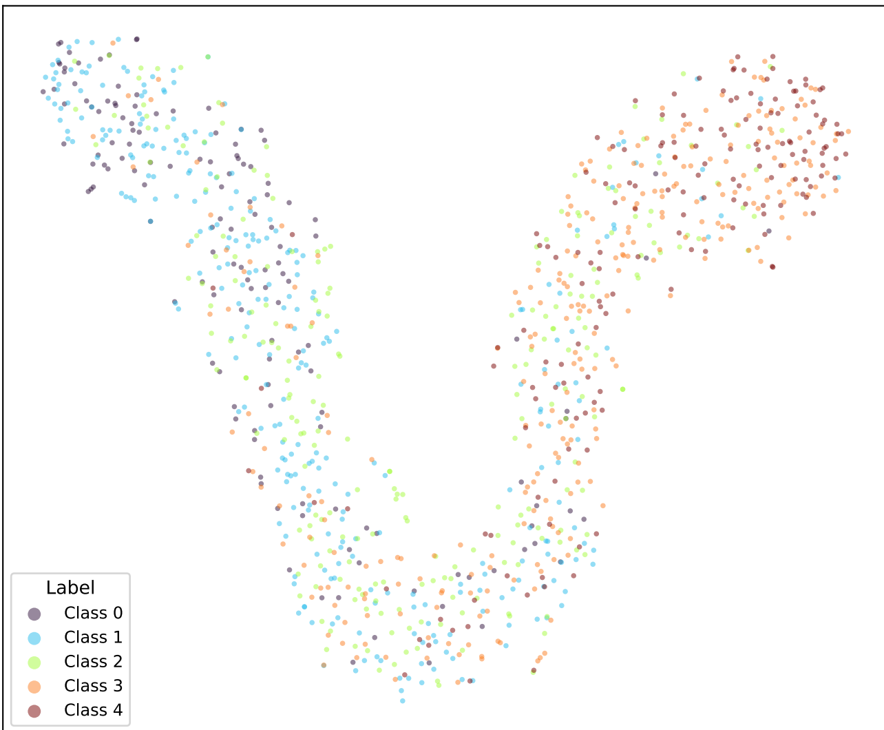
google/bert_uncased_L-2_H-128_A-2-sst5-OLL2-TRIPa2-4 (val)
