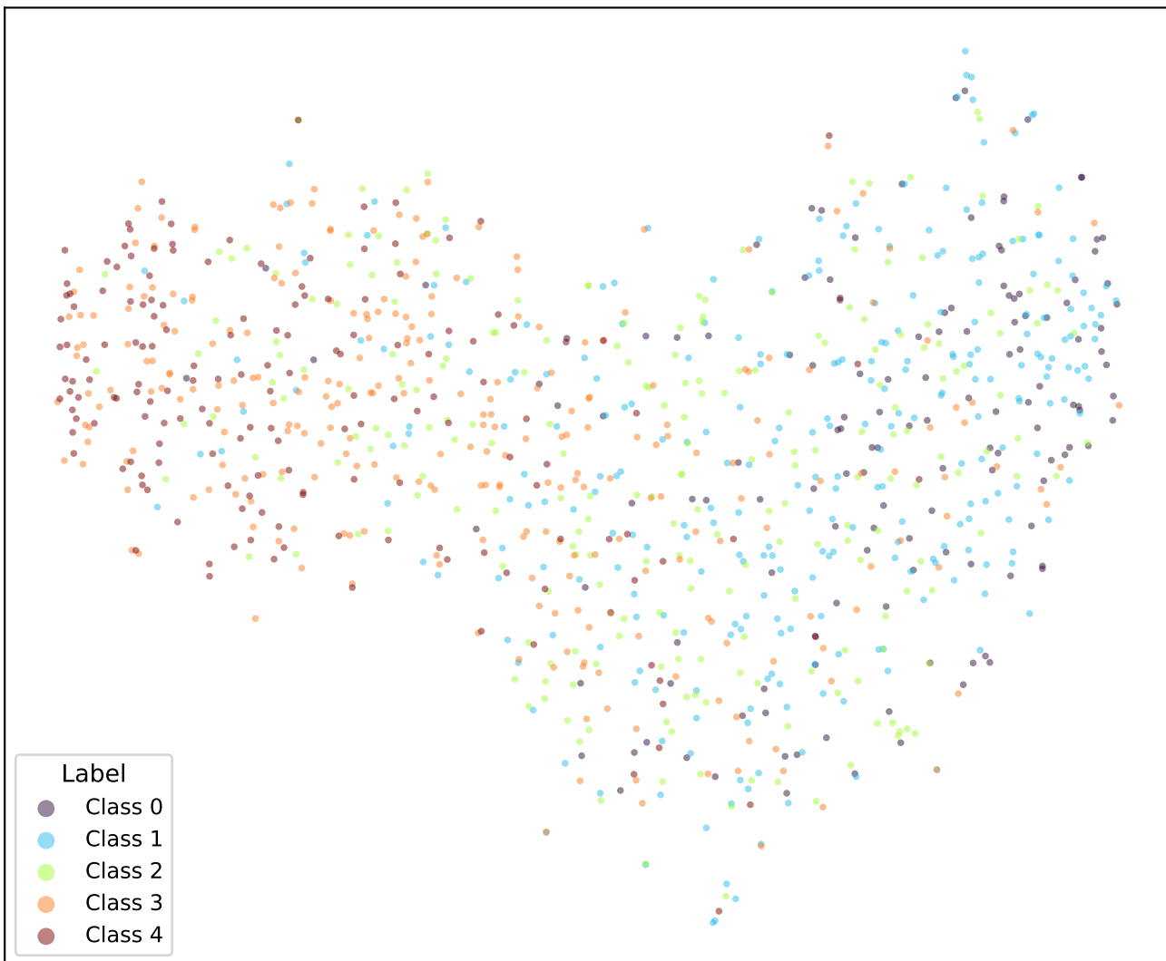
google/bert_uncased_L-2_H-128_A-2-sst5-SOFT2-TRIPa1-3 (val)
