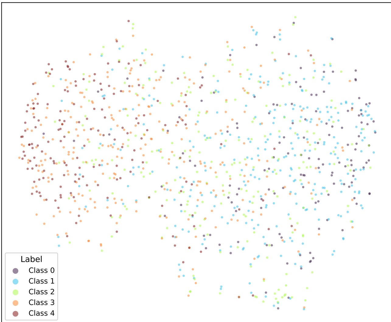
google/bert_uncased_L-2_H-128_A-2-sst5-SOFT2-TRIPa2-1 (val)
