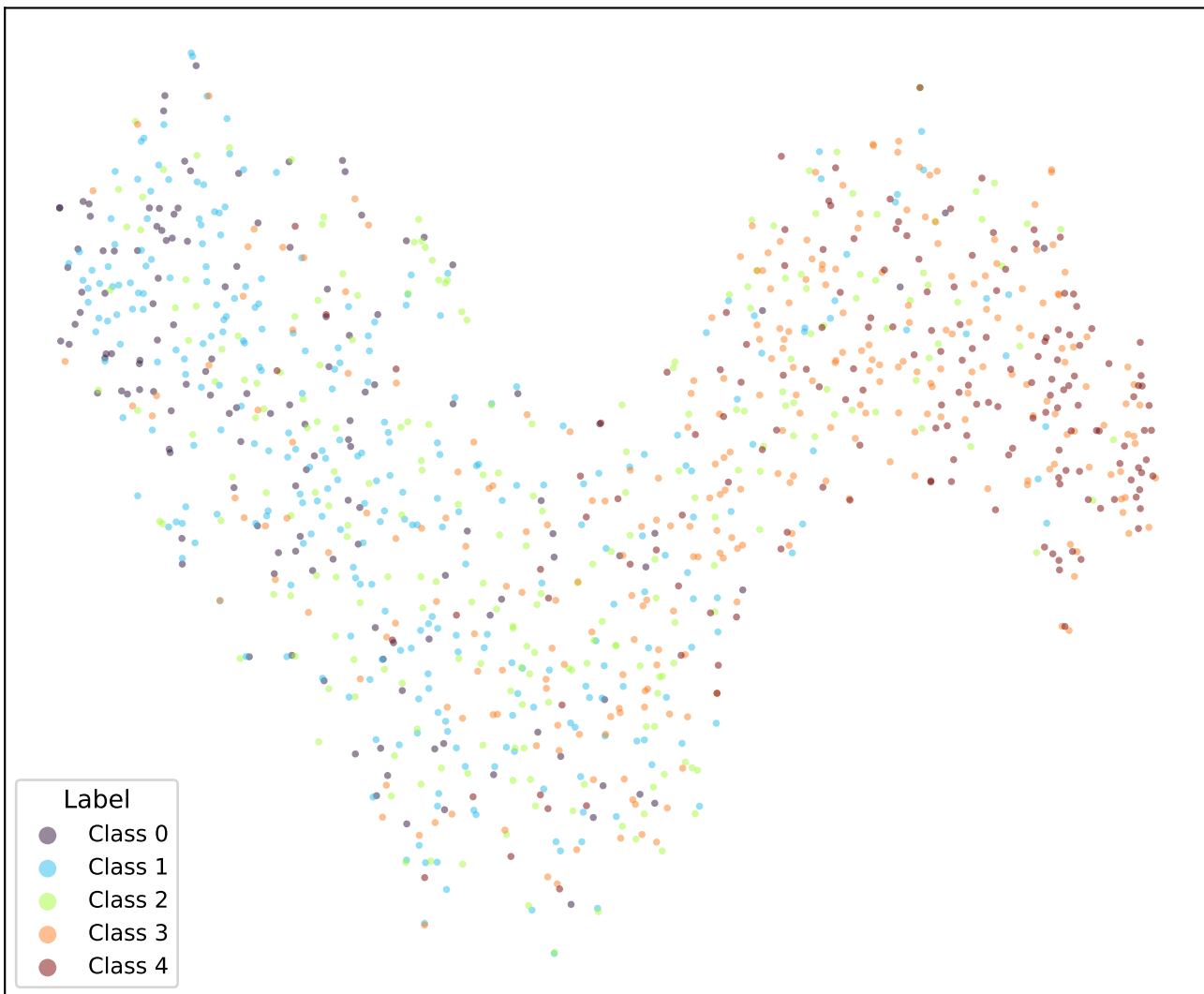
google/bert_uncased_L-2_H-128_A-2-sst5-SOFT2-TRIPa2-3 (val)
