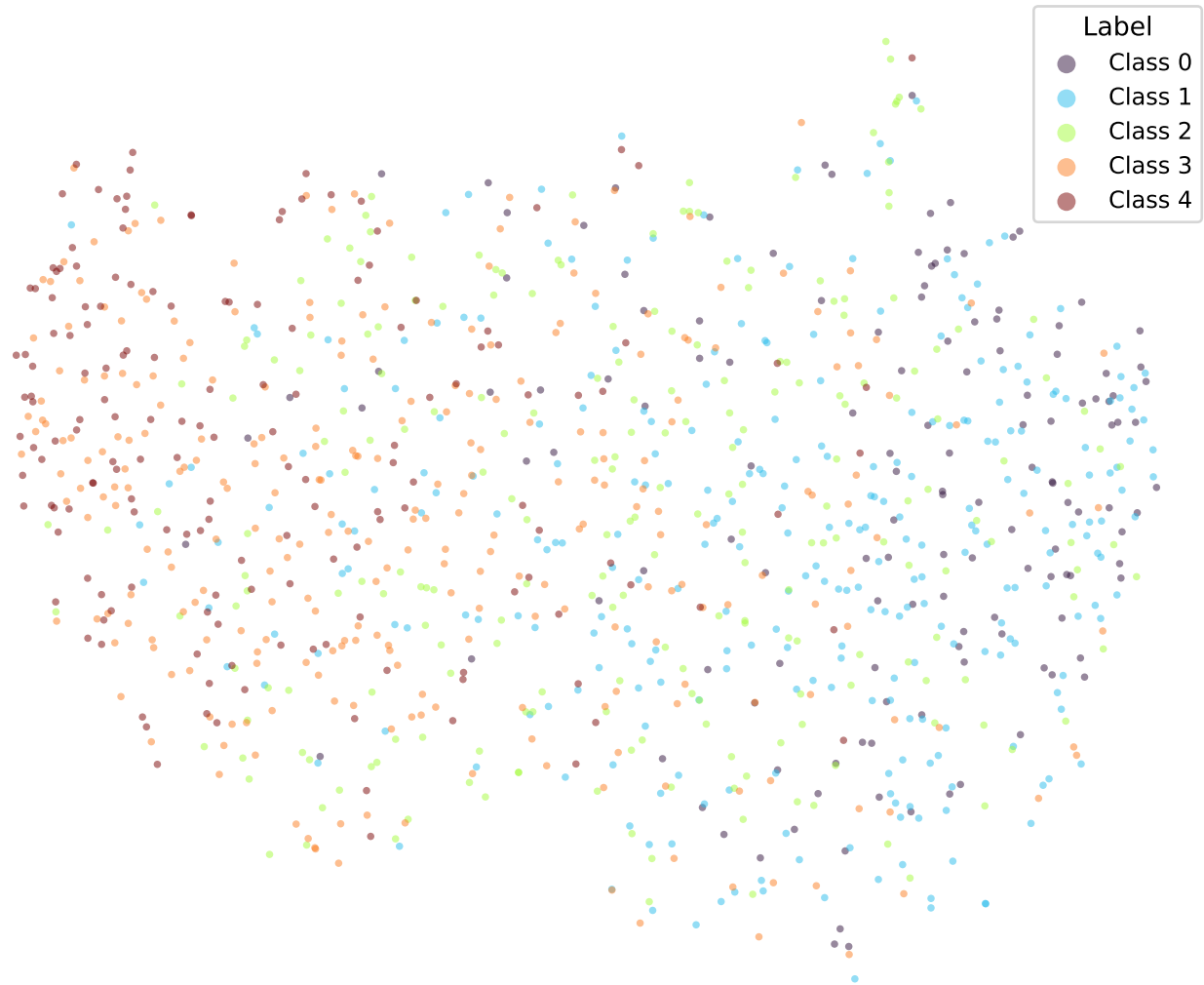
google/bert_uncased_L-2_H-128_A-2-sst5-SOFT2-TRIPa2-4 (val)
