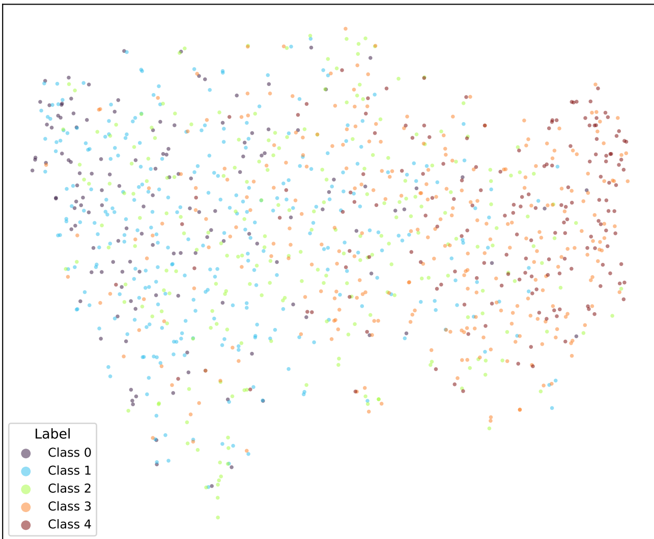
google/bert_uncased_L-2_H-128_A-2-sst5-SOFT3-TRIPa1-1 (val)
