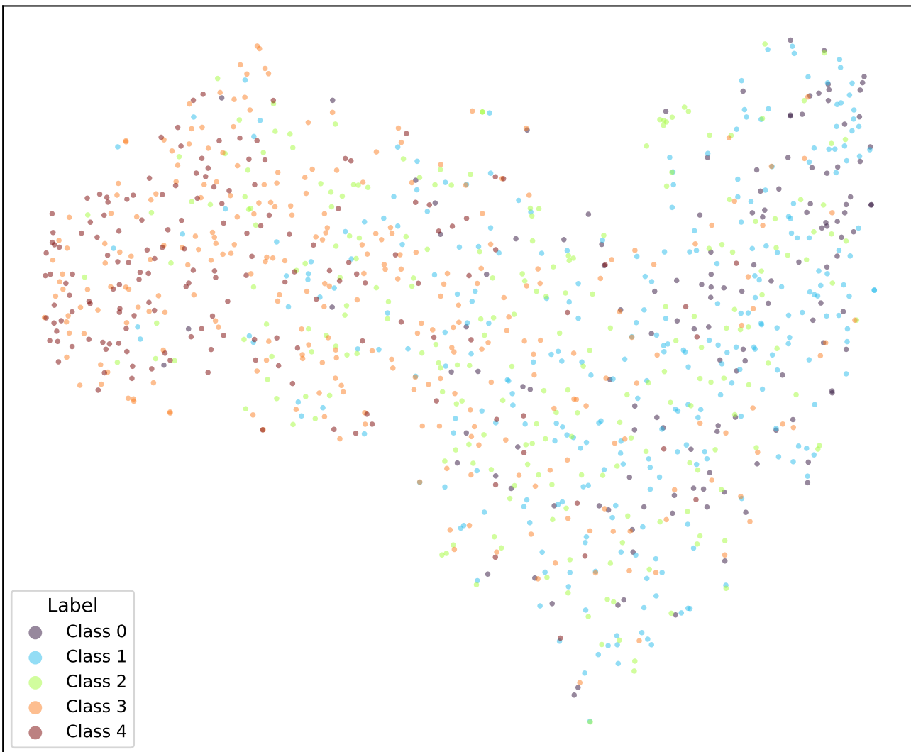
google/bert_uncased_L-2_H-128_A-2-sst5-SOFT3-TRIPa1-3 (val)
