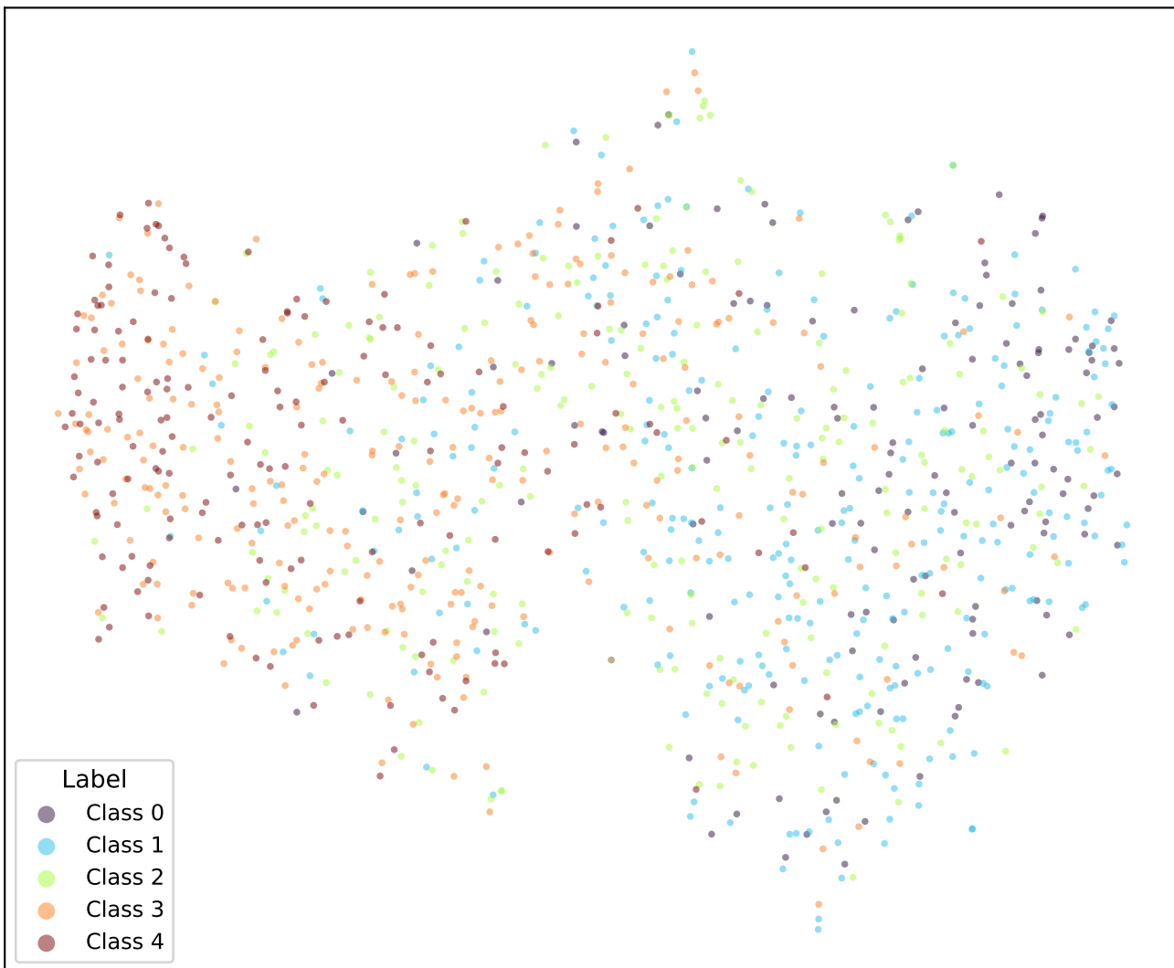
google/bert_uncased_L-2_H-128_A-2-sst5-SOFT3-TRIPa1-4 (val)
