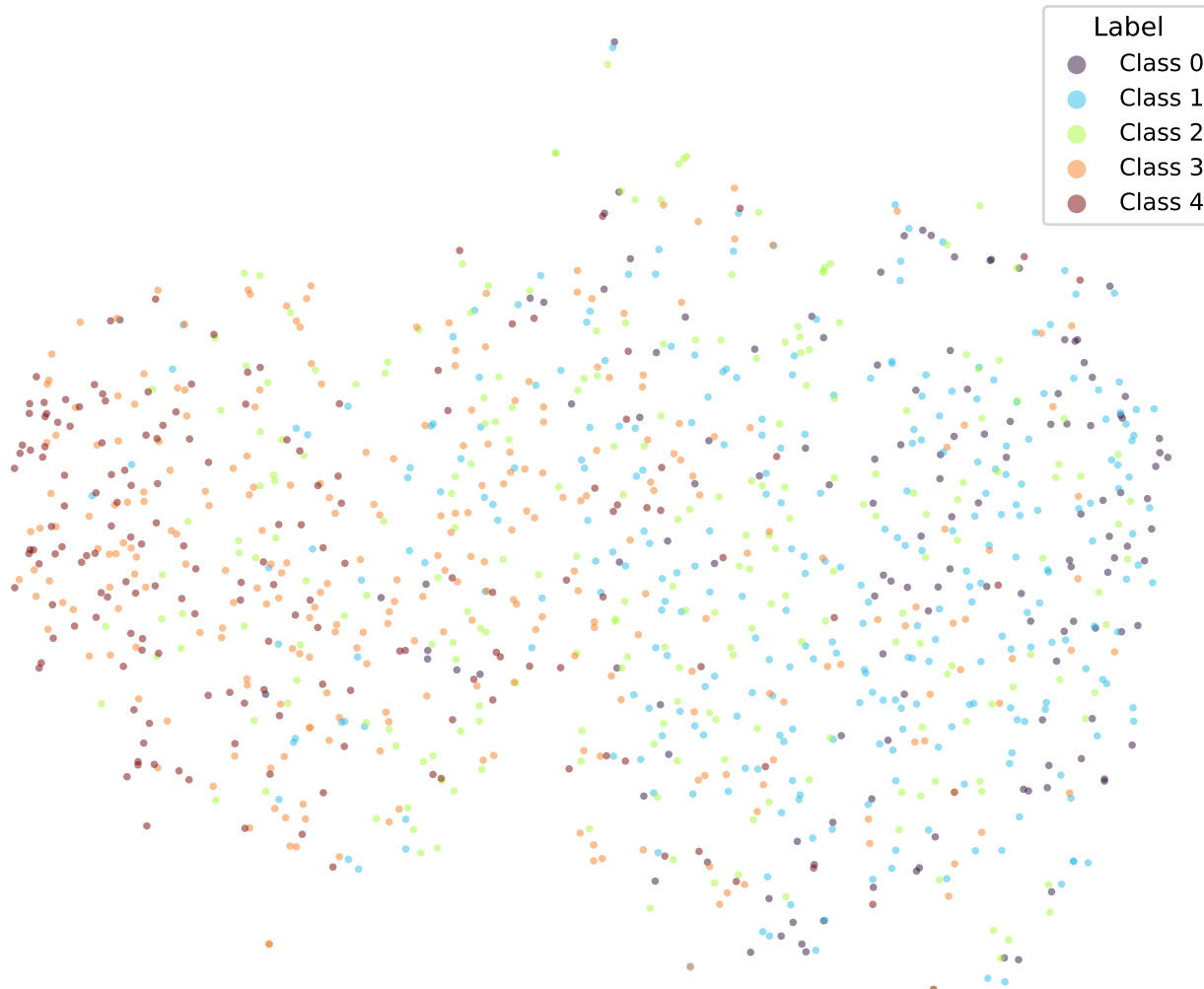
google/bert_uncased_L-2_H-128_A-2-sst5-SOFT3-TRIPa1-5 (val)
