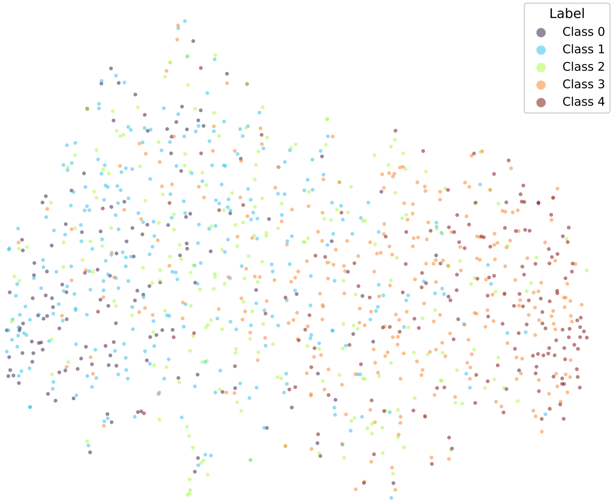
google/bert_uncased_L-2_H-128_A-2-sst5-SOFT3-TRIPa2-2 (val)
