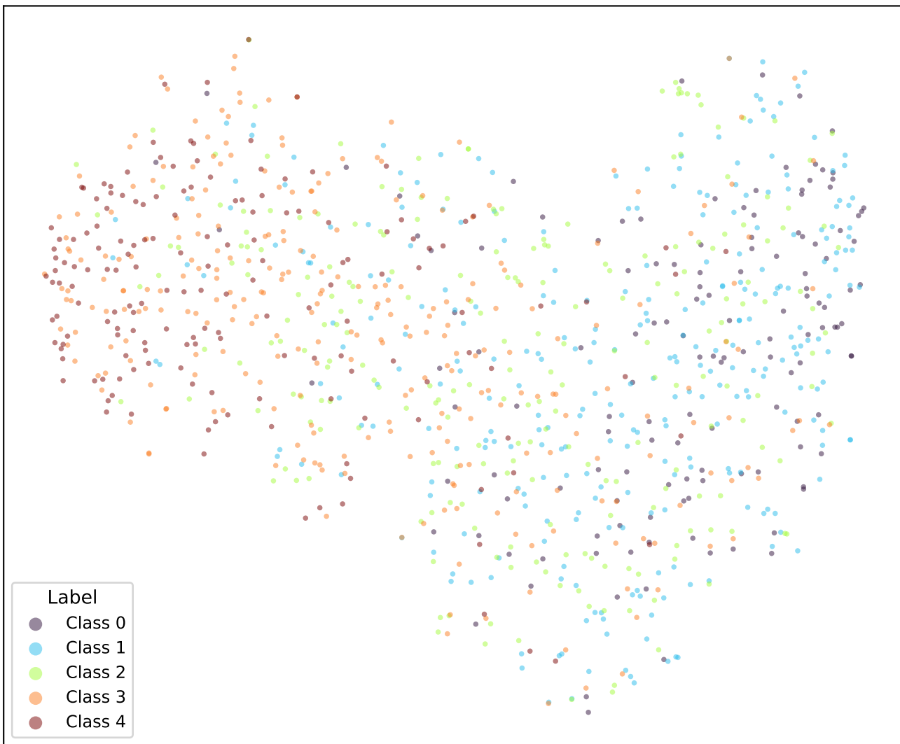
google/bert_uncased_L-2_H-128_A-2-sst5-SOFT3-TRIPa2-3 (val)
