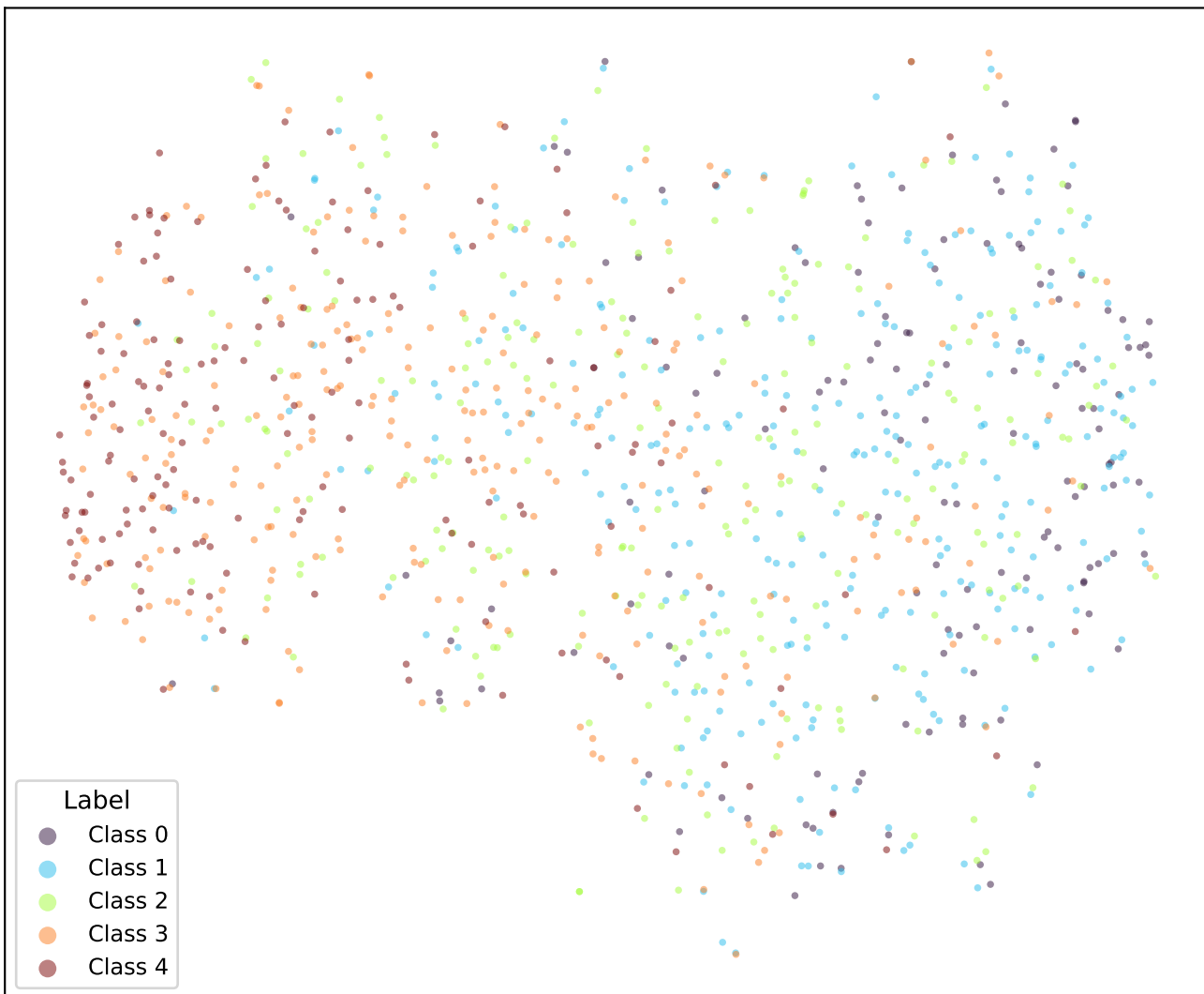
google/bert_uncased_L-2_H-128_A-2-sst5-SOFT3-TRIPa2-5 (val)
