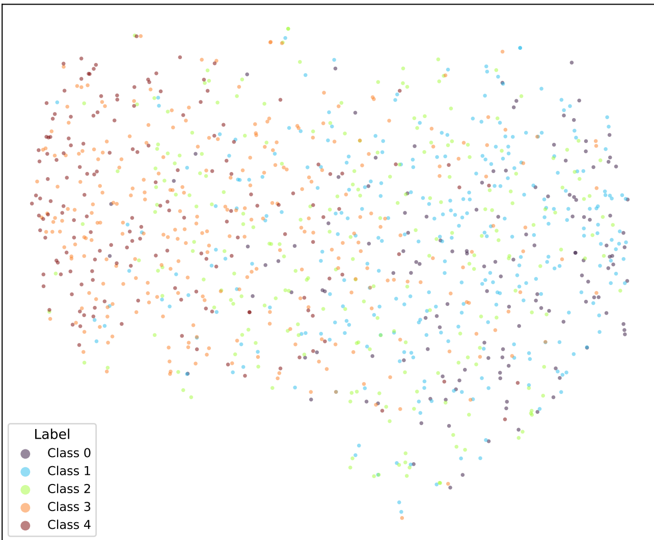
google/bert_uncased_L-2_H-128_A-2-sst5-SOFT4-TRIPa1-4 (val)
