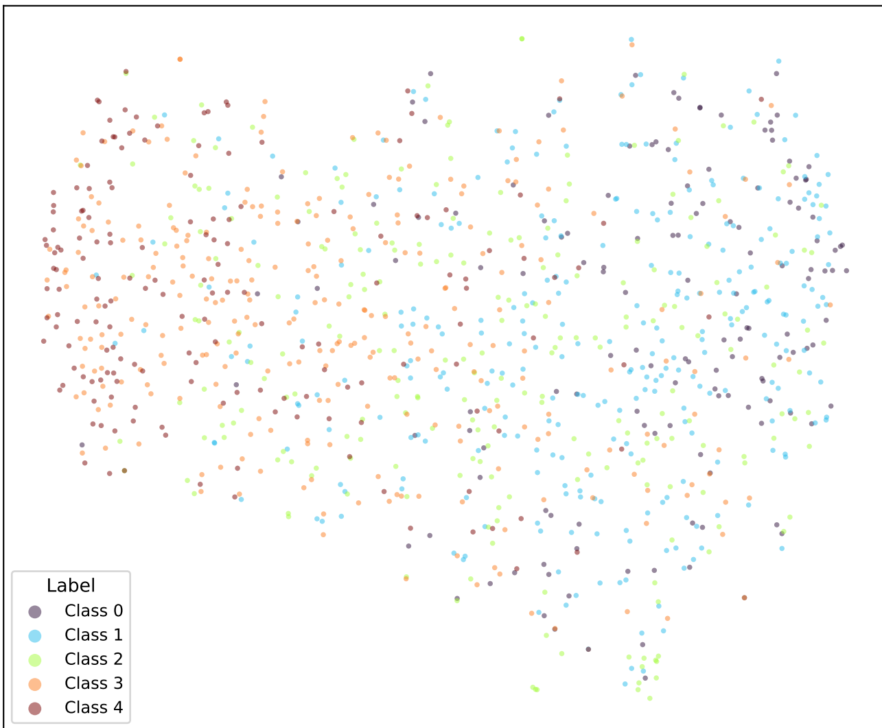
google/bert_uncased_L-2_H-128_A-2-sst5-SOFT4-TRIPa1-5 (val)
