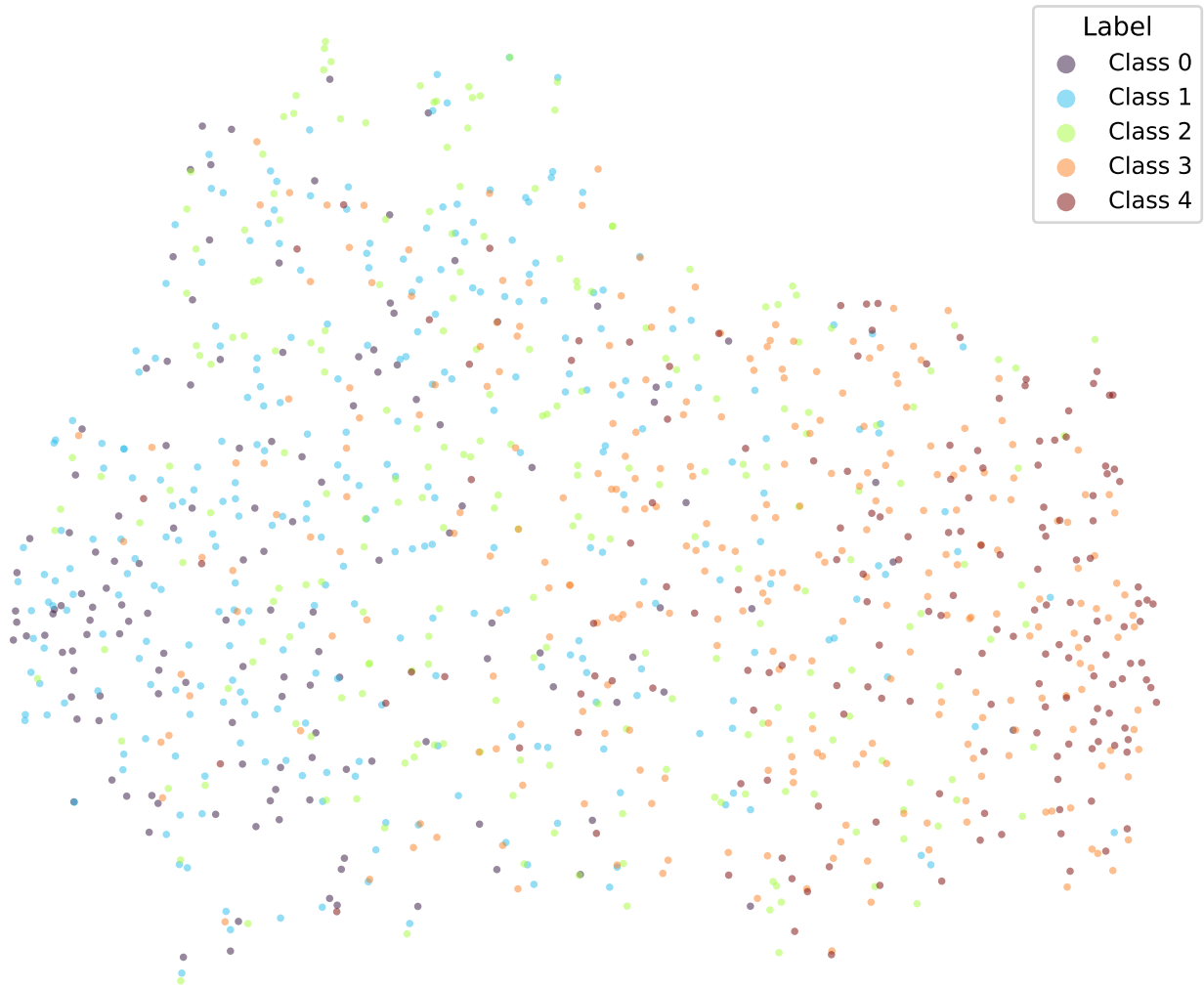
google/bert_uncased_L-2_H-128_A-2-sst5-SOFT4-TRIPa2-2 (val)
